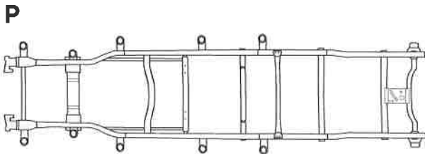
UNDERBODY VIEW
