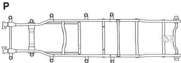
UNDERBODY VIEW
